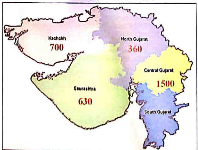
Figure 4: Per capita water availability in Gujarat in cubic meters/year (in 2011)
